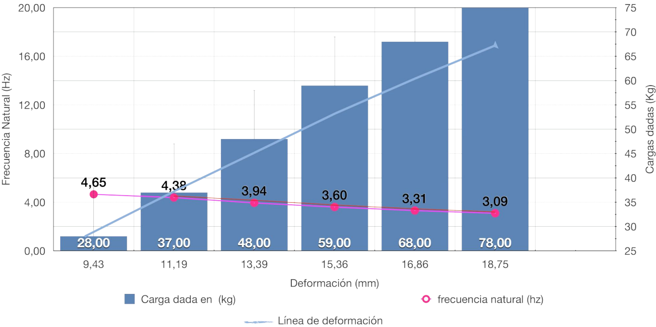
Laboratory Test UNE-EN ISO 10846-1:2009
